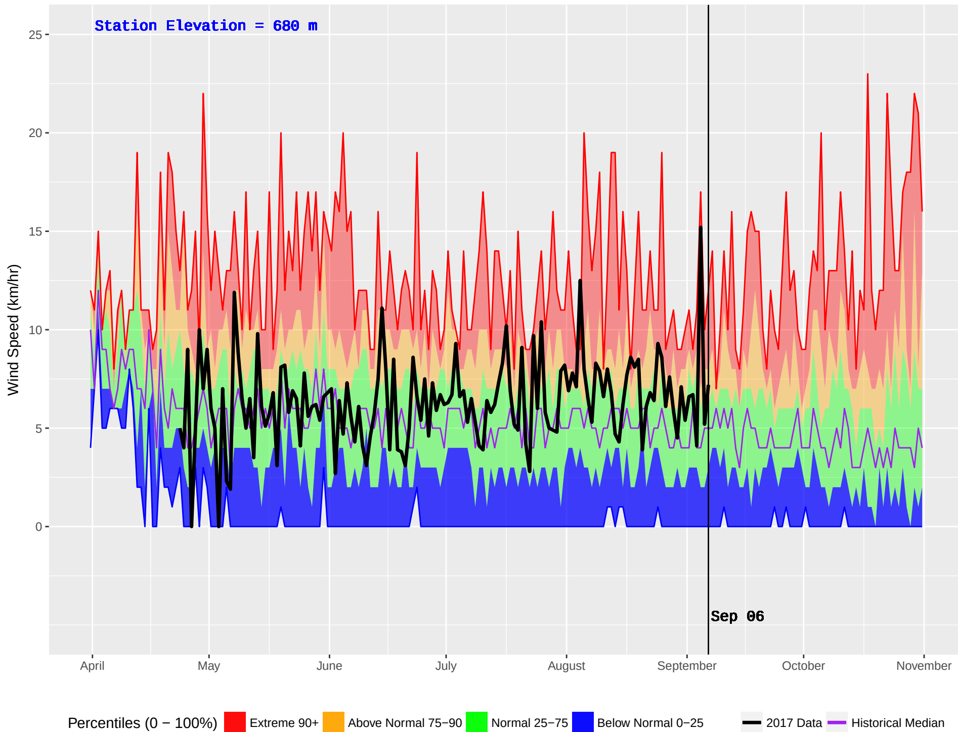
REVELSTOKE (363) : Historical (1995–2016) and Current (2017) Noon Wind Speed
